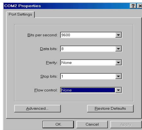
Figure 4.1 - Communication Parameters
