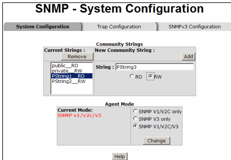
Figure 5.29 – SNMP Management
