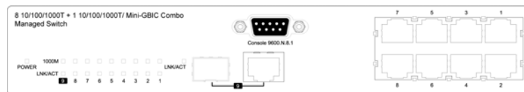
Figure 3.2 - Front Panel of the GSM2109 Switch
