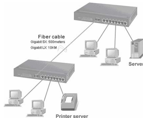
Figure 4-3 Use fiber port to extend the distance between workgroups
