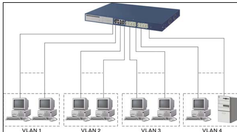
Figure 3-4 - Port-based VLAN Diagram
