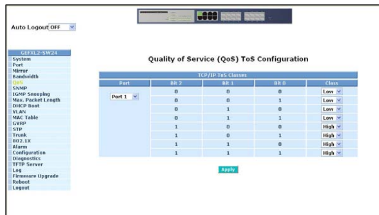
Figure 5.20 – QoS ToS Configuration
