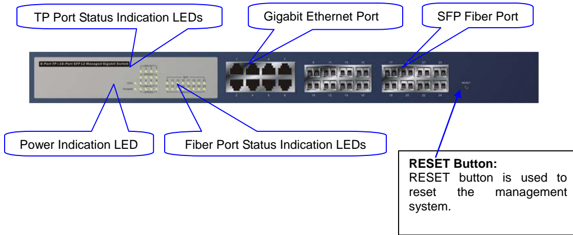
Figure 3-1 - Front View of GSM2824
